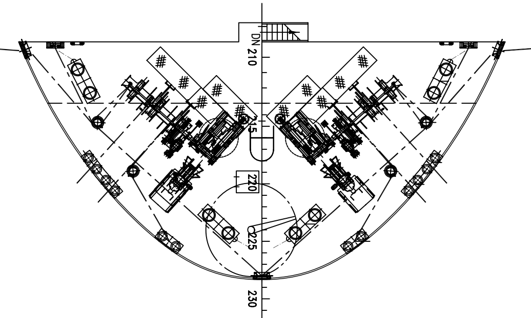
PRINCIPAL PARTICULARS
